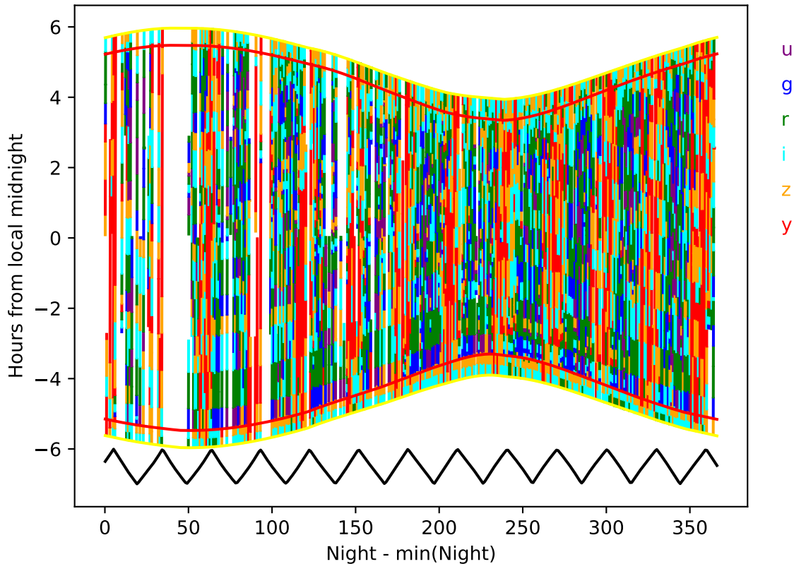
too_combined_s0.0_v3.4_10yrs year 6-7: Hourglass
