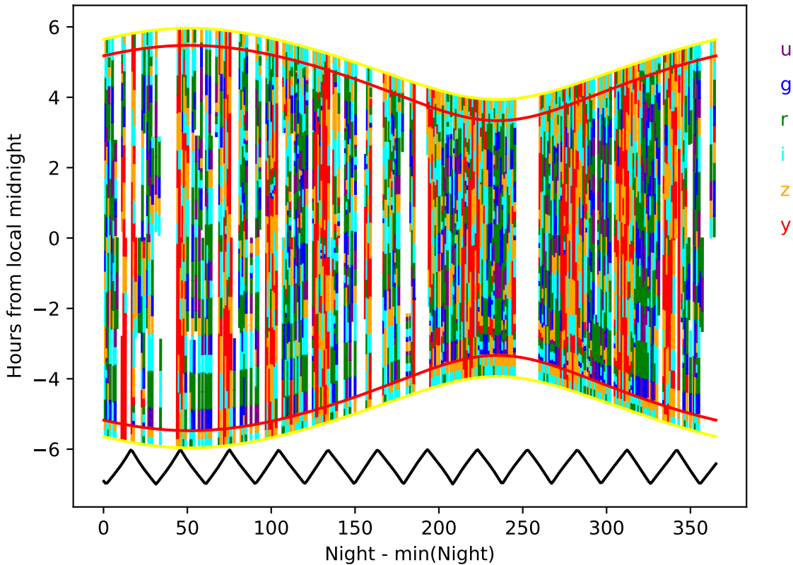
too_combined_s0.0_v3.4_10yrs year 5-6: Hourglass
