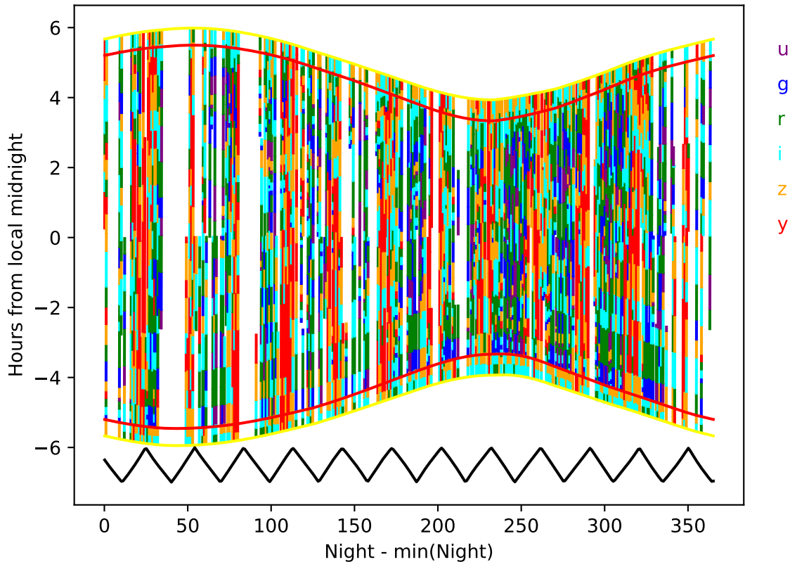
too_combined_s0.0_v3.4_10yrs year 4-5: Hourglass
