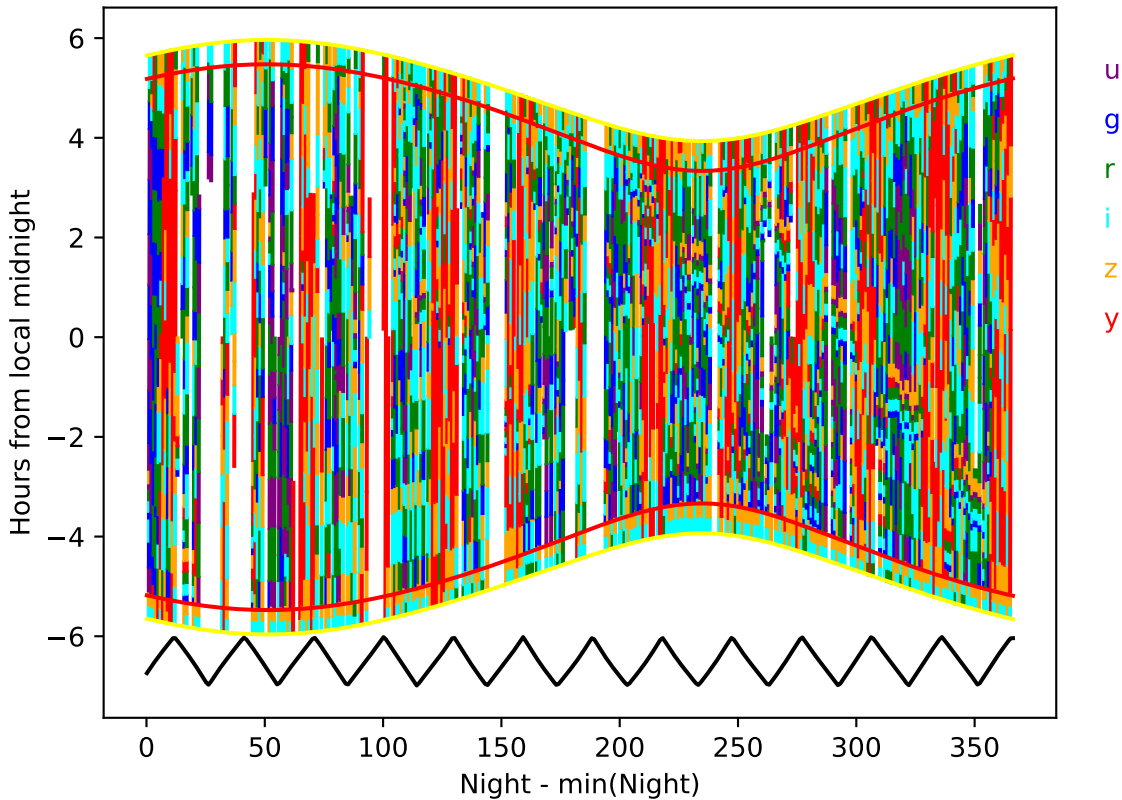
too_combined_s0.0_v3.4_10yrs year 0-1: Hourglass
