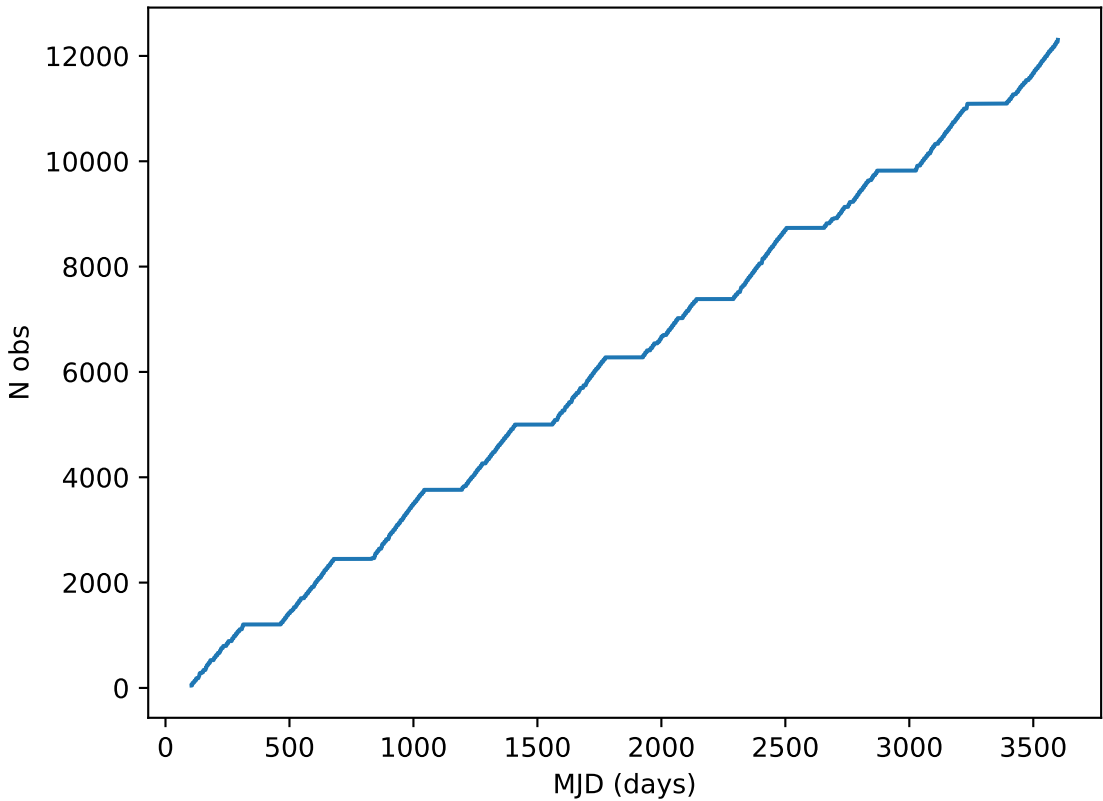
too_combined_s0.0_v3.4_10yrs note like DD:EDFS_b%: Cumulative
