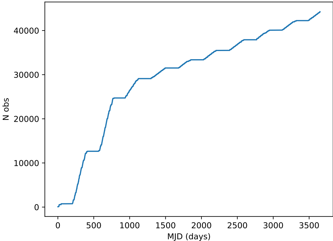
too_combined_s0.0_v3.4_10yrs note like DD:COSMOS%: Cumulative
