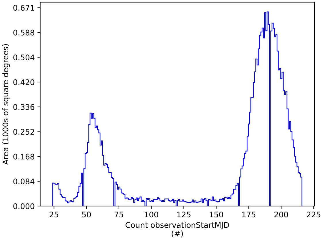
too_combined_s0.0_v3.4_10yrs i: Count observationStartMJD
