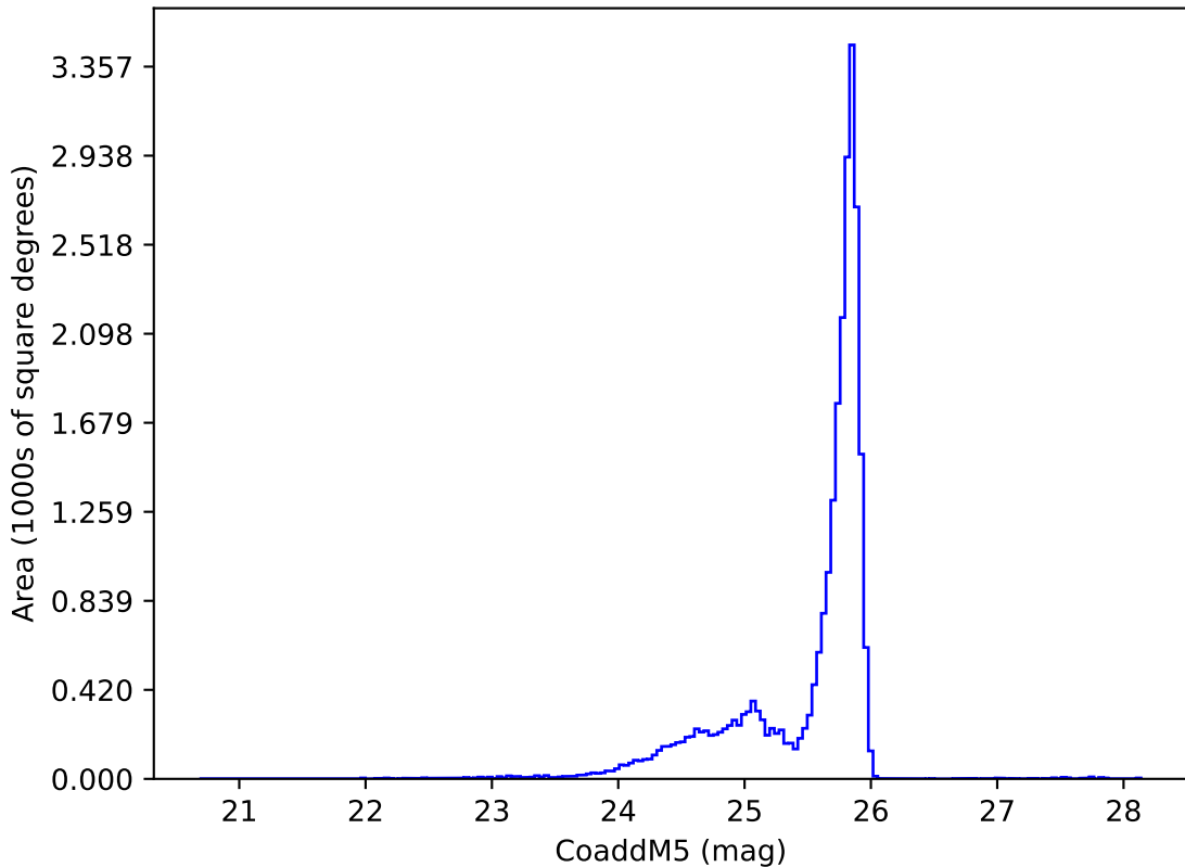
too_combined_s0.0_v3.4_10yrs z: CoaddM5
