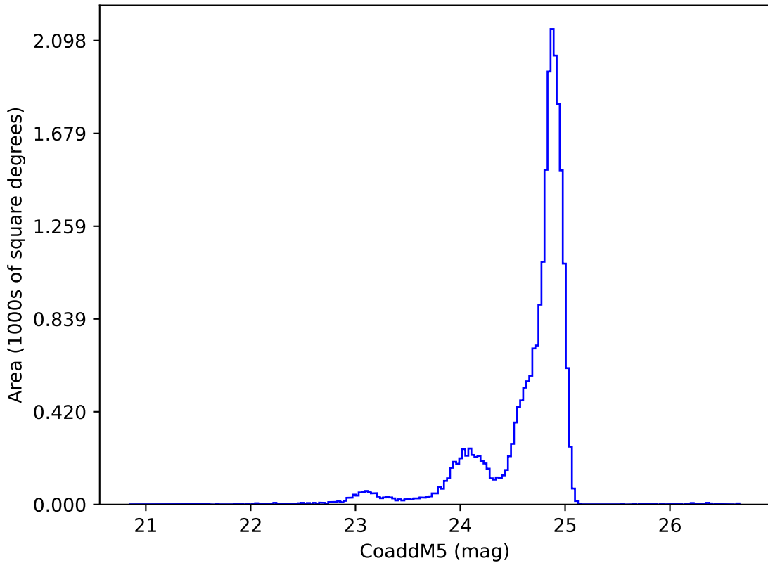
too_combined_s0.0_v3.4_10yrs y: CoaddM5
