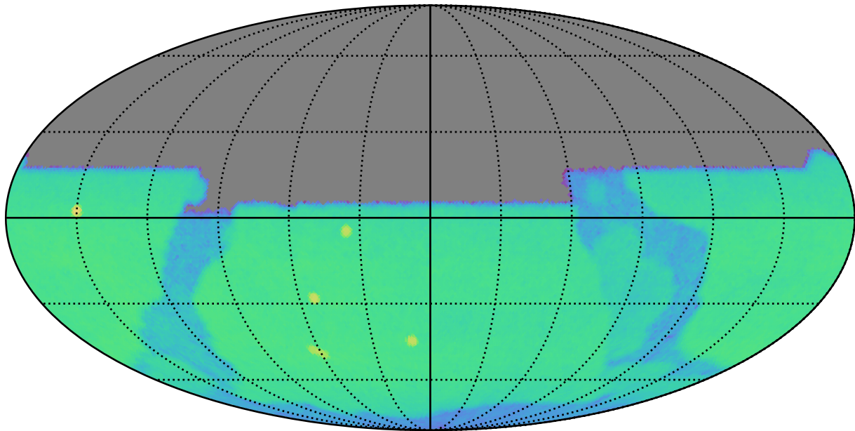
too_combined_s0.0_v3.4_10yrs u: CoaddM5
