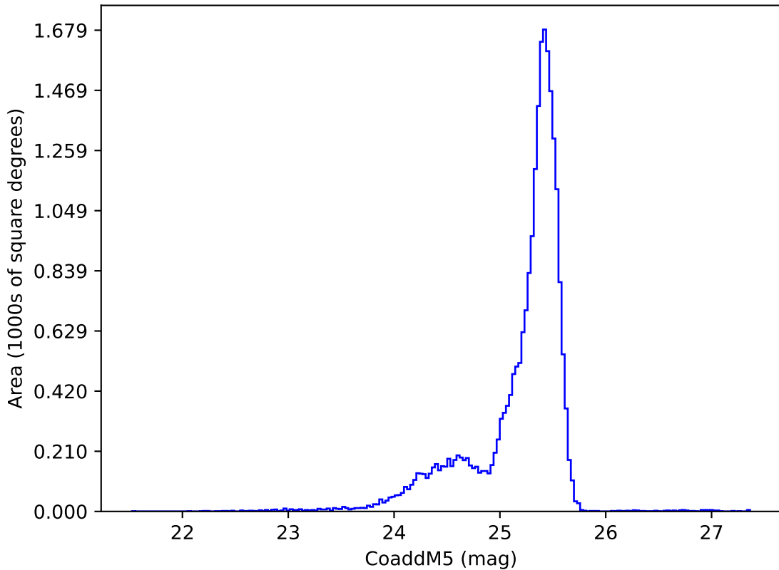
too_combined_s0.0_v3.4_10yrs u: CoaddM5
