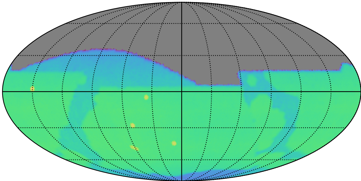
too_combined_s0.0_v3.4_10yrs r: CoaddM5
