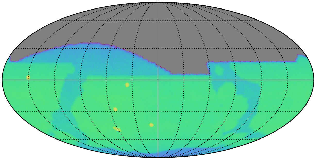
too_combined_s0.0_v3.4_10yrs i: CoaddM5
