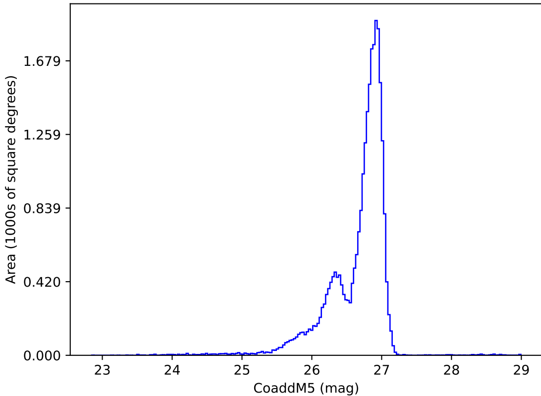
too_combined_s0.0_v3.4_10yrs g: CoaddM5
