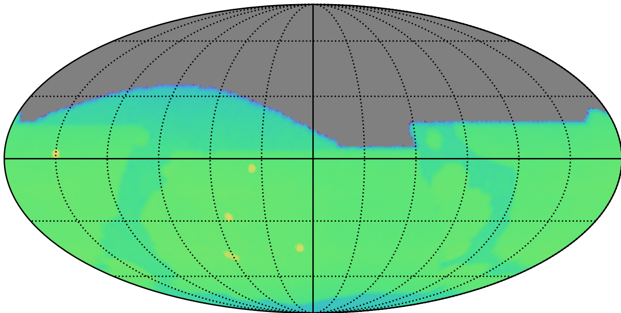
too_combined_s0.0_v3.4_10yrs : CoaddM5
