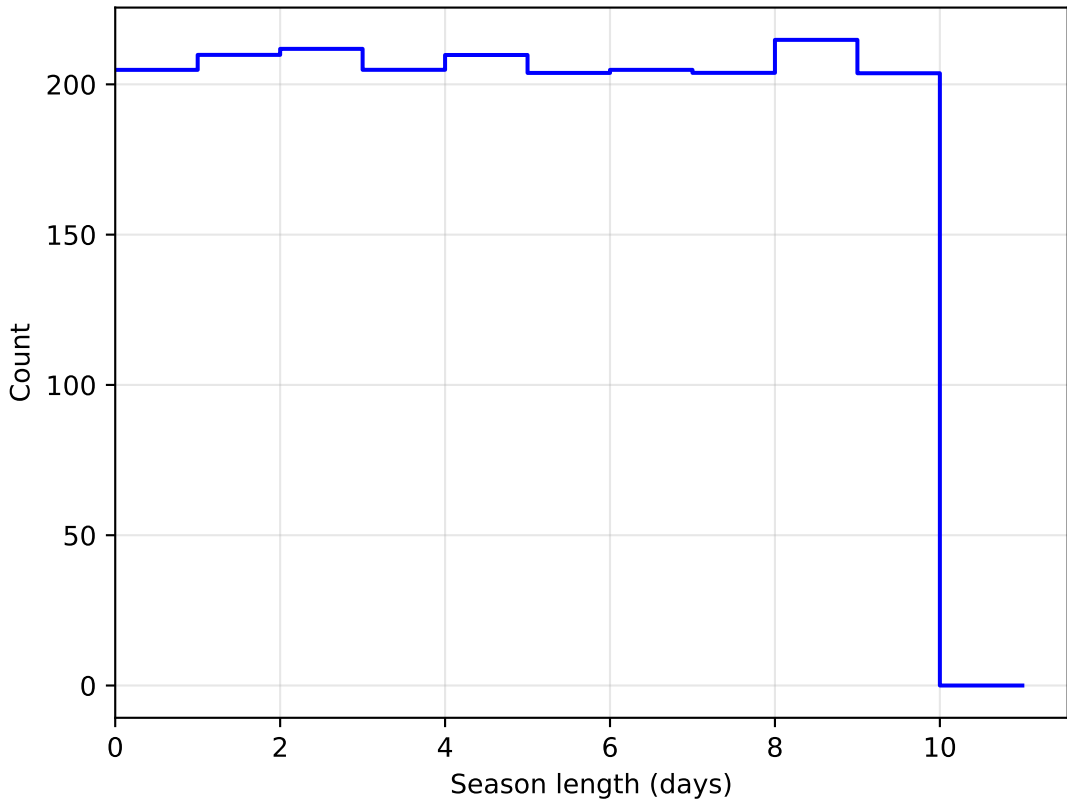
too_combined_s0.0_v3.4_10yrs DD:ECDFS all bands: SeasonLength
