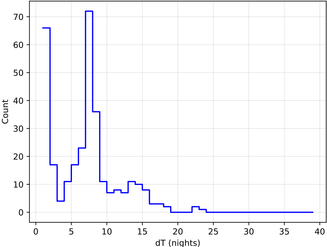
too_combined_s0.0_v3.4_10yrs all bands: DD:XMM_LSS Delta Nights Histogram
