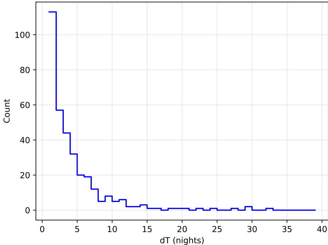
too_combined_s0.0_v3.4_10yrs all bands: DD:WFD Delta Nights Histogram
