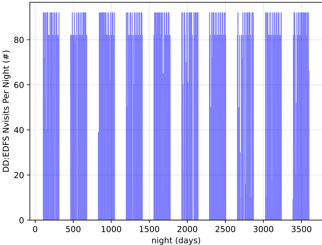
too_combined_s0.0_v3.4_10yrs all bands: DD:EDFS Nvisits Per Night
