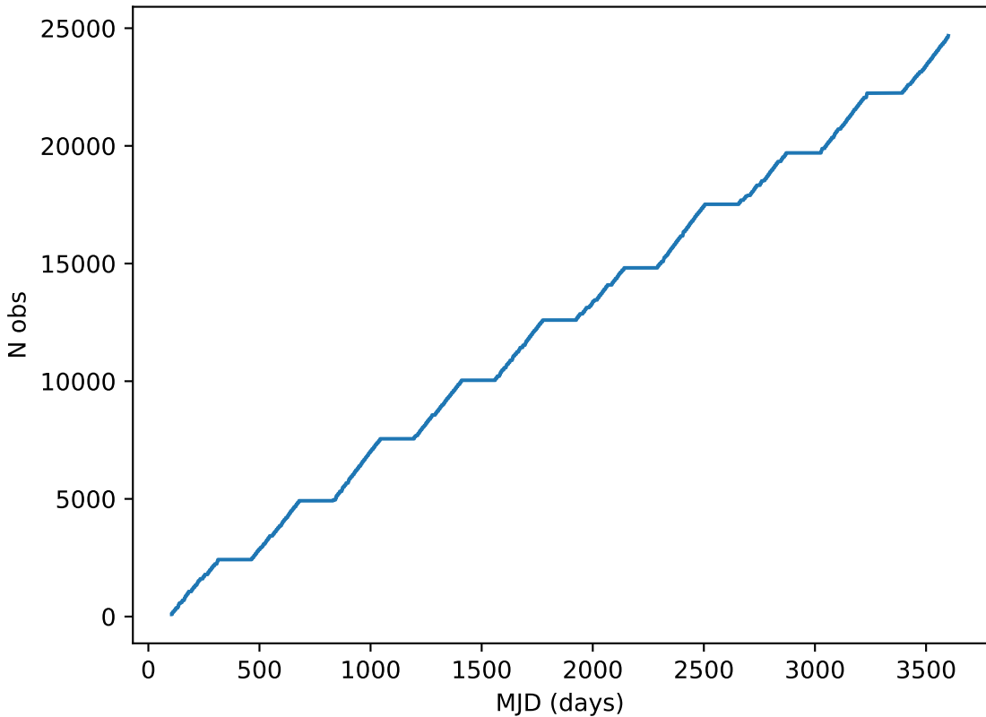
too_combined_s0.0_v3.4_10yrs all bands: DD:EDFS Cumulative NVisits
