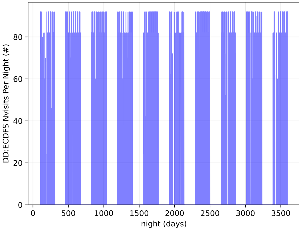
too_combined_s0.0_v3.4_10yrs all bands: DD:ECDFS Nvisits Per Night
