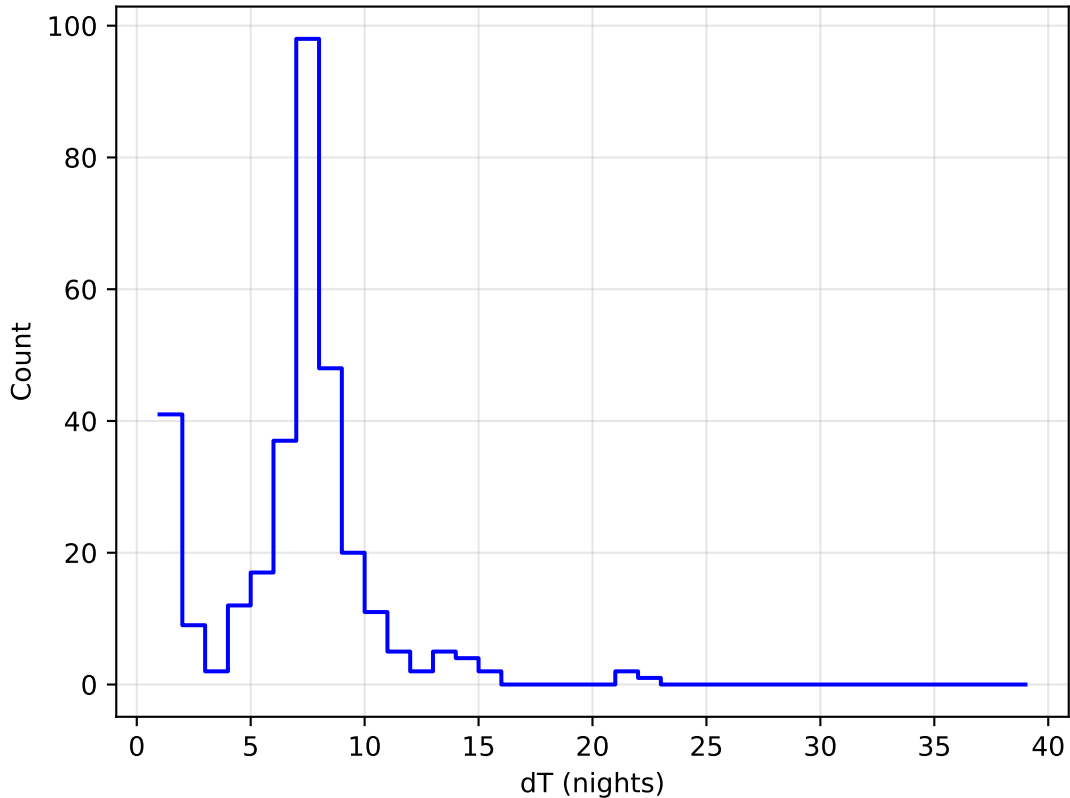
too_combined_s0.0_v3.4_10yrs all bands: DD:ECDFS Delta Nights Histogram
