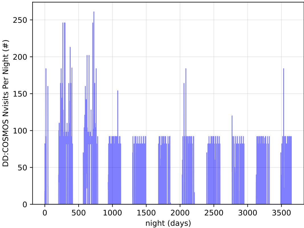
too_combined_s0.0_v3.4_10yrs all bands: DD:COSMOS Nvisits Per Night
