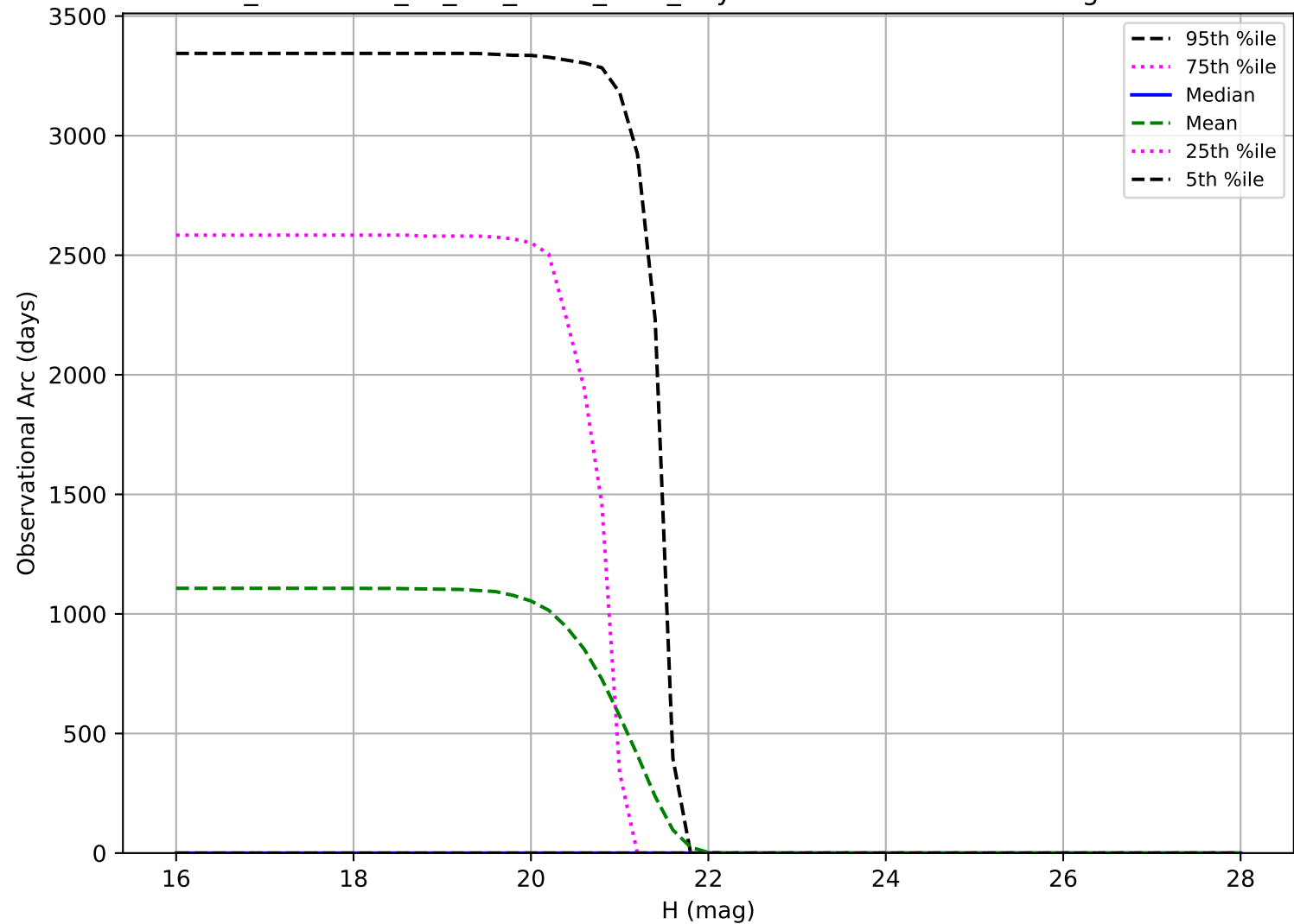
too_combined_no_nss_s10.0_v3.4_10yrs: Observational Arc Length Vatira
