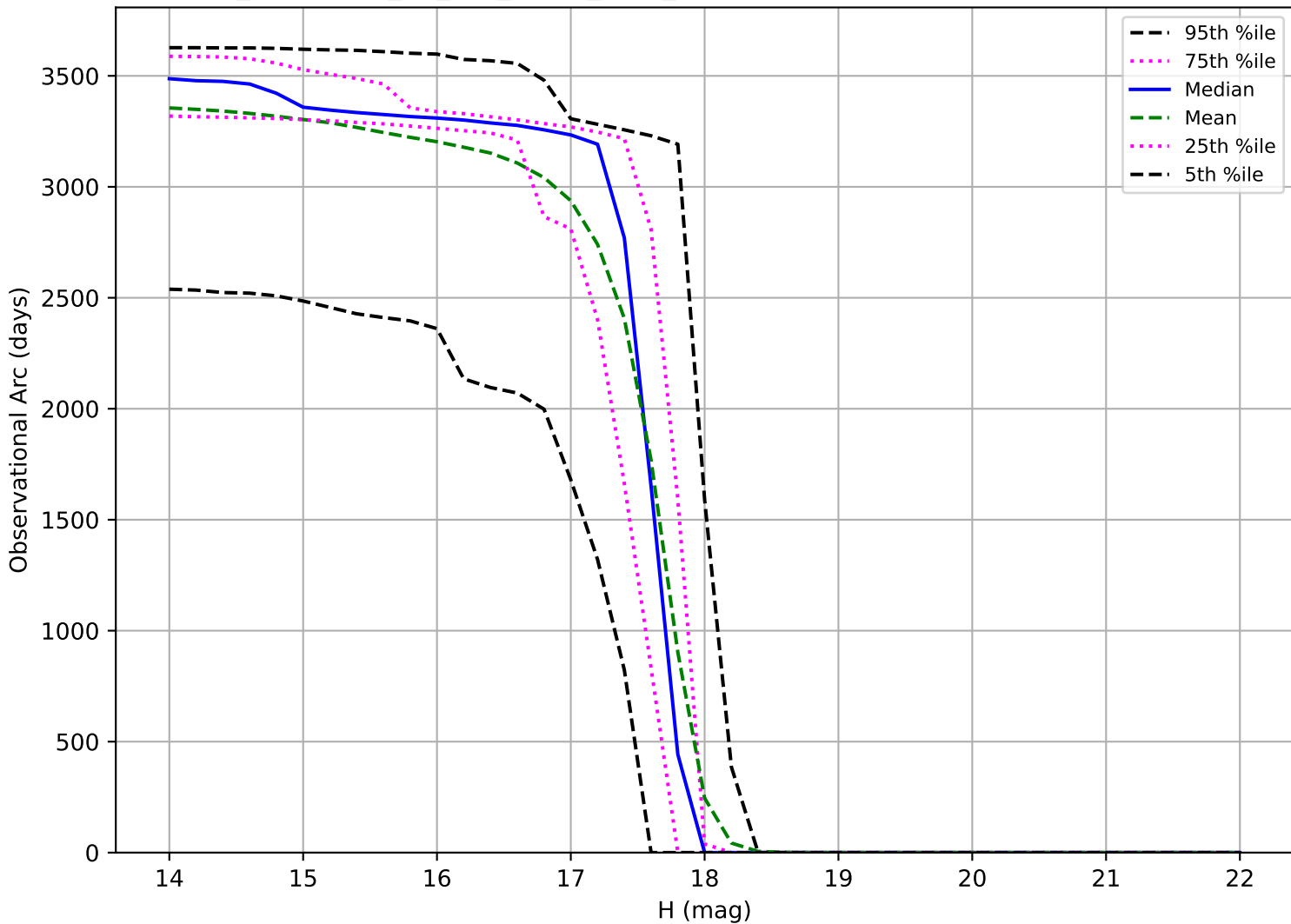
too_combined_no_nss_s10.0_v3.4_10yrs: Observational Arc Length Trojan
