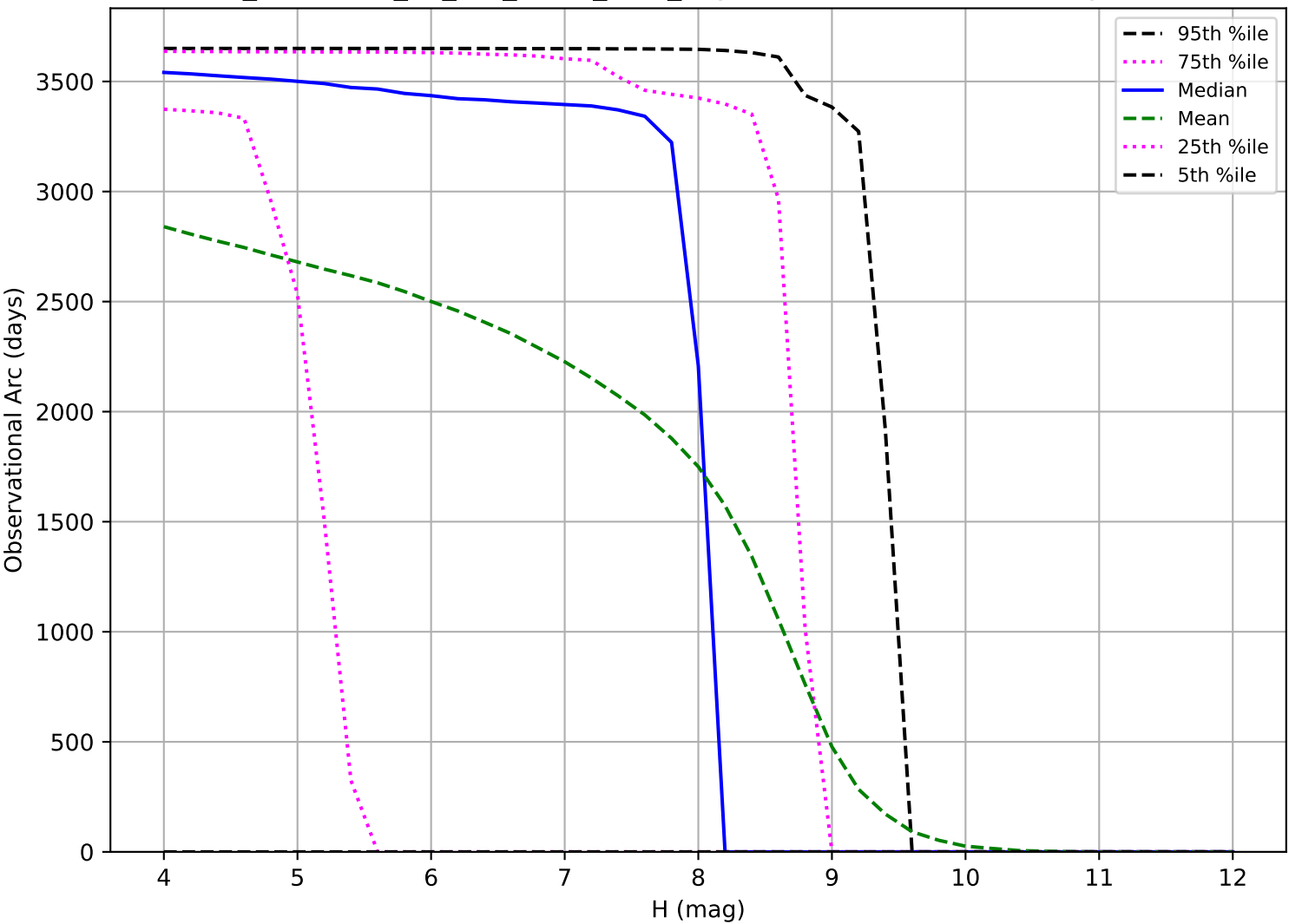
too_combined_no_nss_s10.0_v3.4_10yrs: Observational Arc Length TNO
