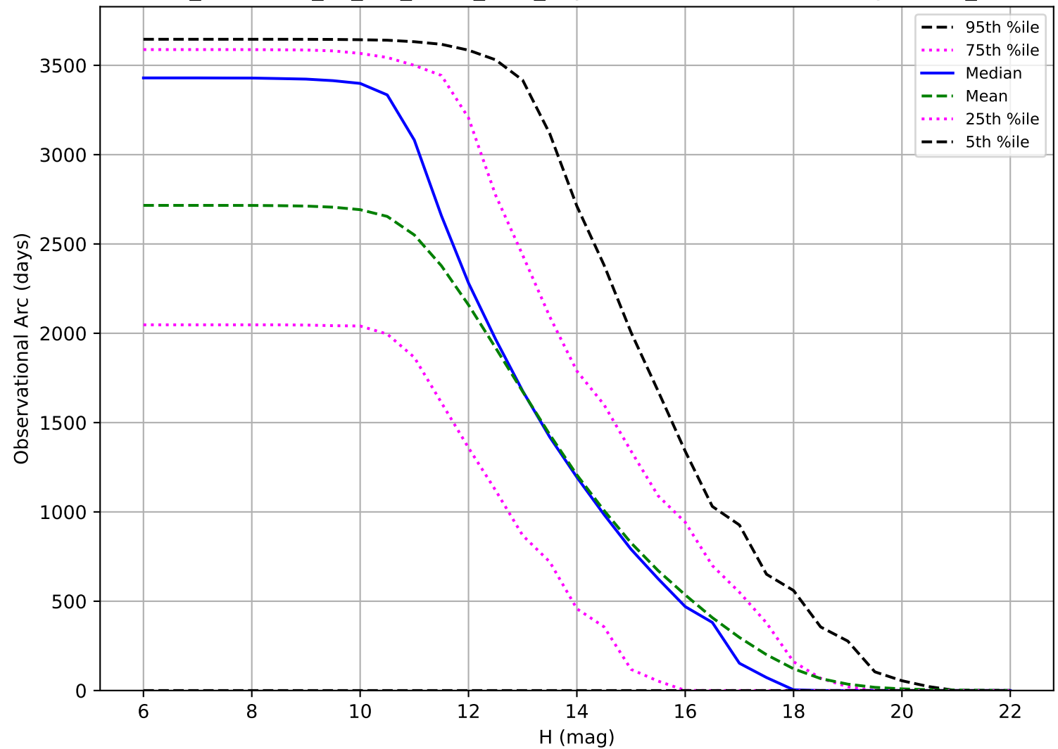
too_combined_no_nss_s10.0_v3.4_10yrs: Observational Arc Length OCC_r5
