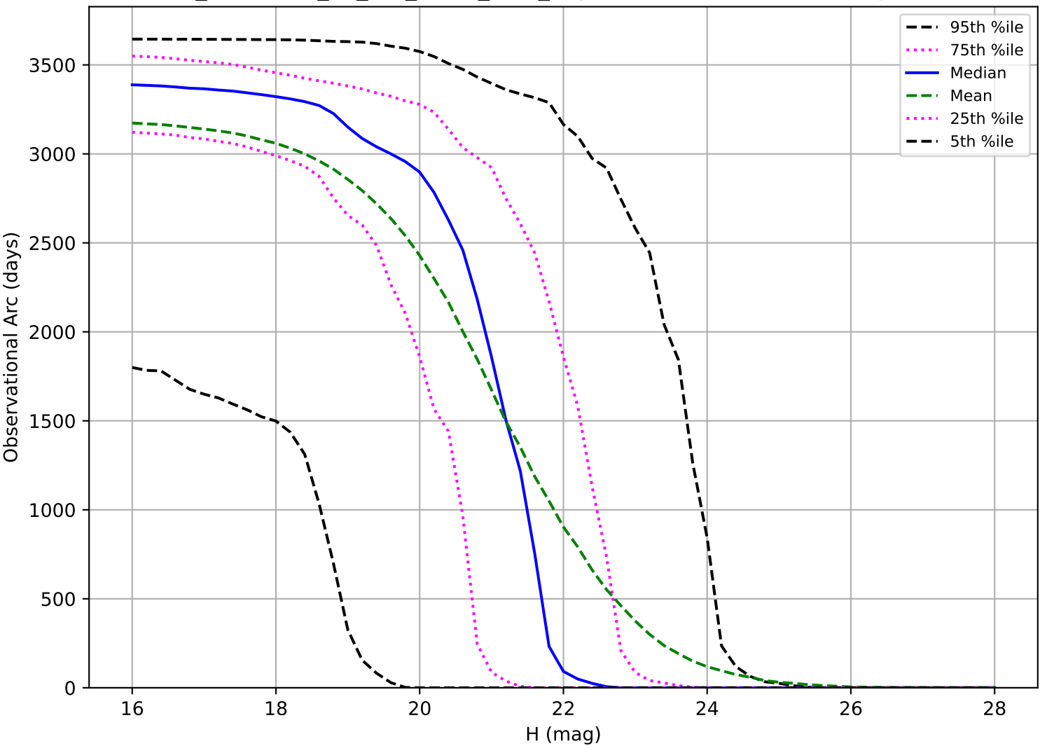
too_combined_no_nss_s10.0_v3.4_10yrs: Observational Arc Length NEO
