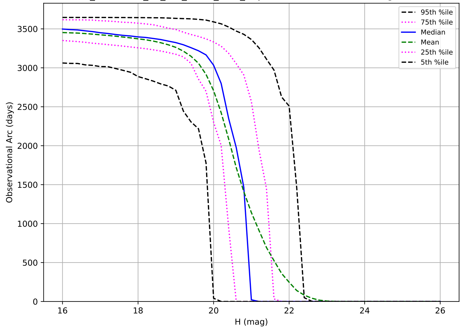
too_combined_no_nss_s10.0_v3.4_10yrs: Observational Arc Length MBA
