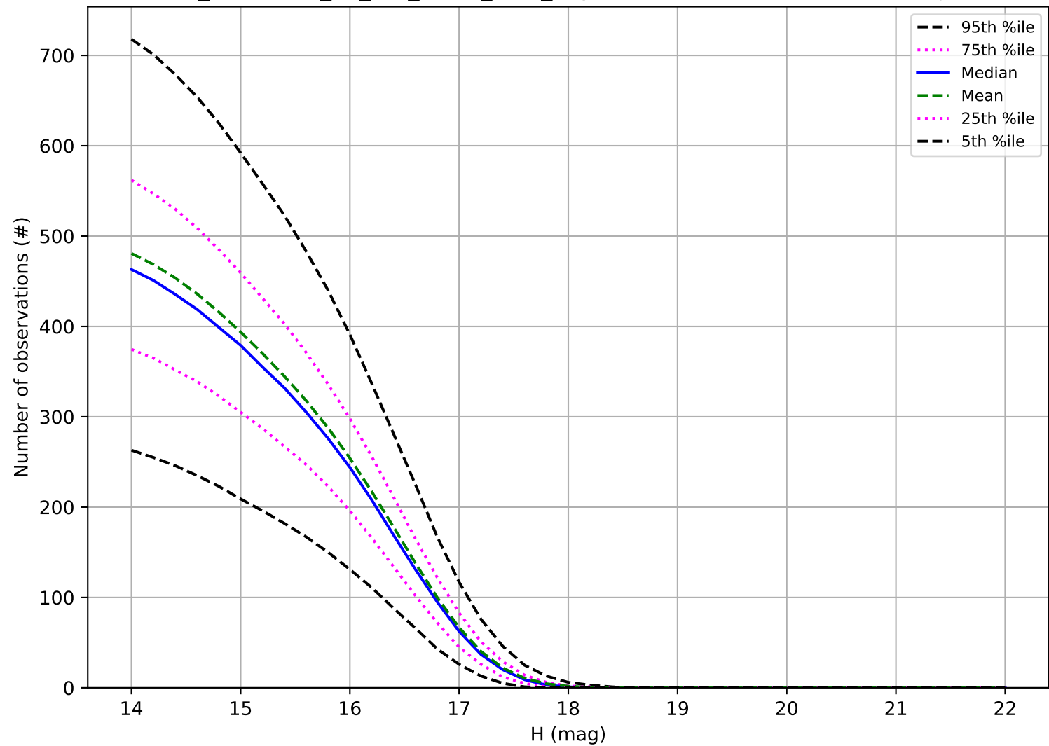
too_combined_no_nss_s10.0_v3.4_10yrs: Number of observations Trojan
