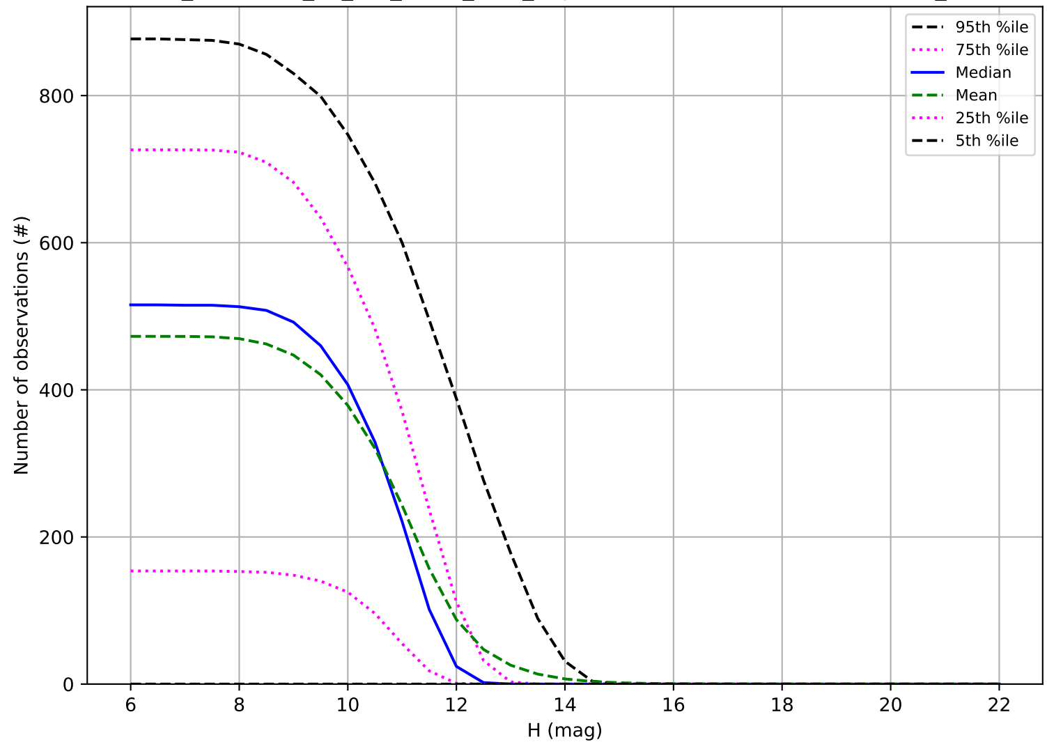
too_combined_no_nss_s10.0_v3.4_10yrs: Number of observations OCC_r20
