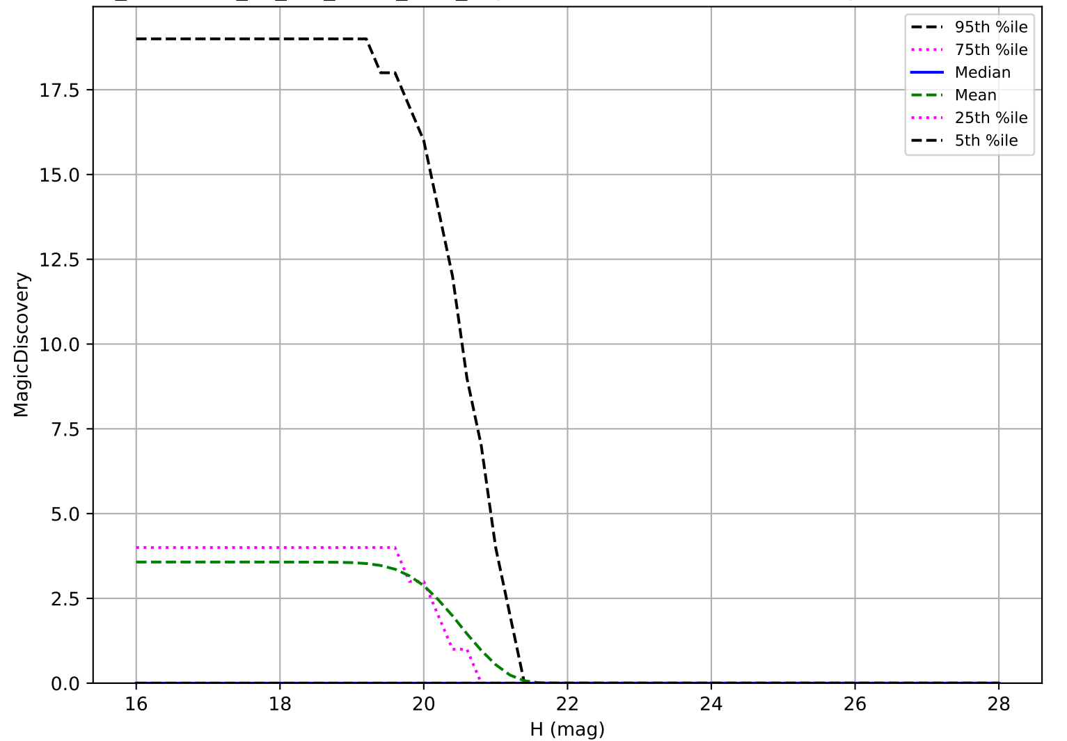
too_combined_no_nss_s10.0_v3.4_10yrs: Vatira 6 detections in 60 nights detection loss
