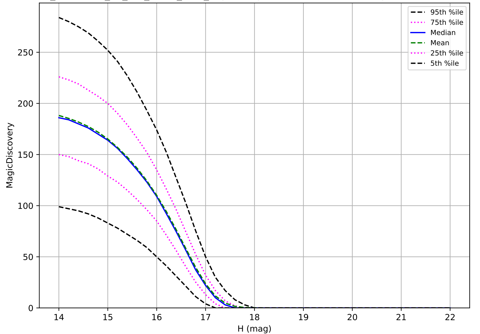
too_combined_no_nss_s10.0_v3.4_10yrs: Trojan 6 detections in 60 nights detection loss
