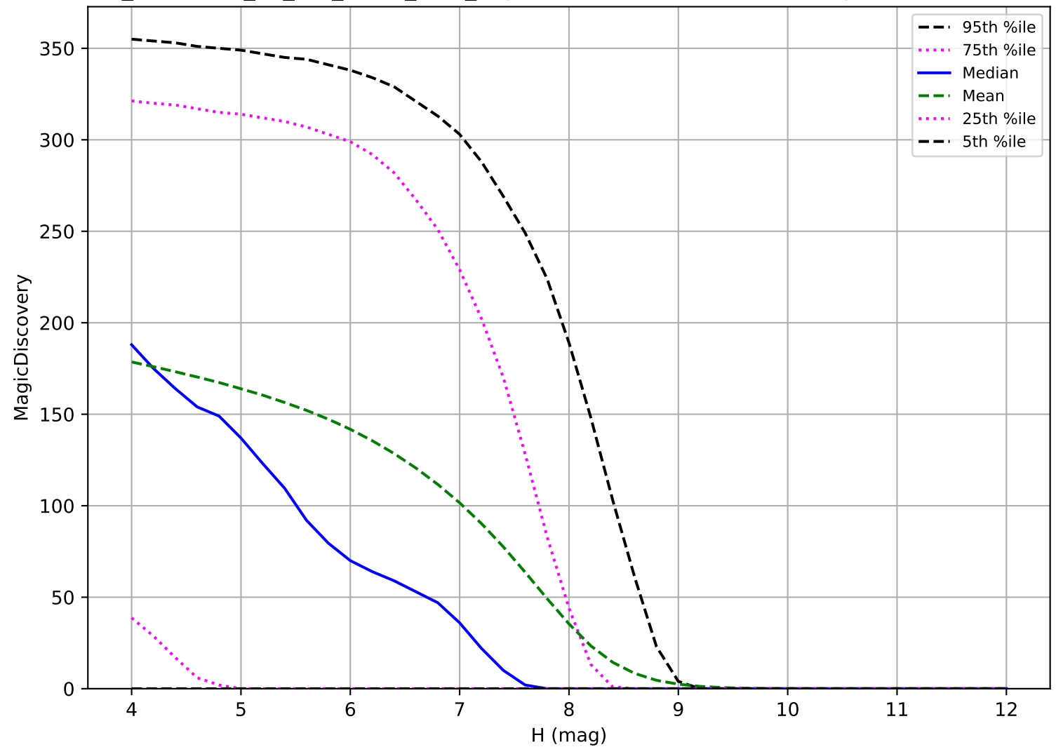
too_combined_no_nss_s10.0_v3.4_10yrs: TNO 6 detections in 60 nights detection loss
