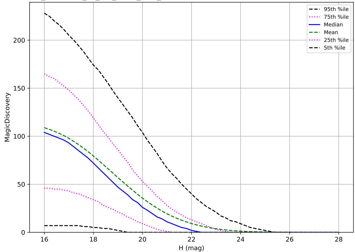
too_combined_no_nss_s10.0_v3.4_10yrs: PHA 6 detections in 60 nights detection loss
