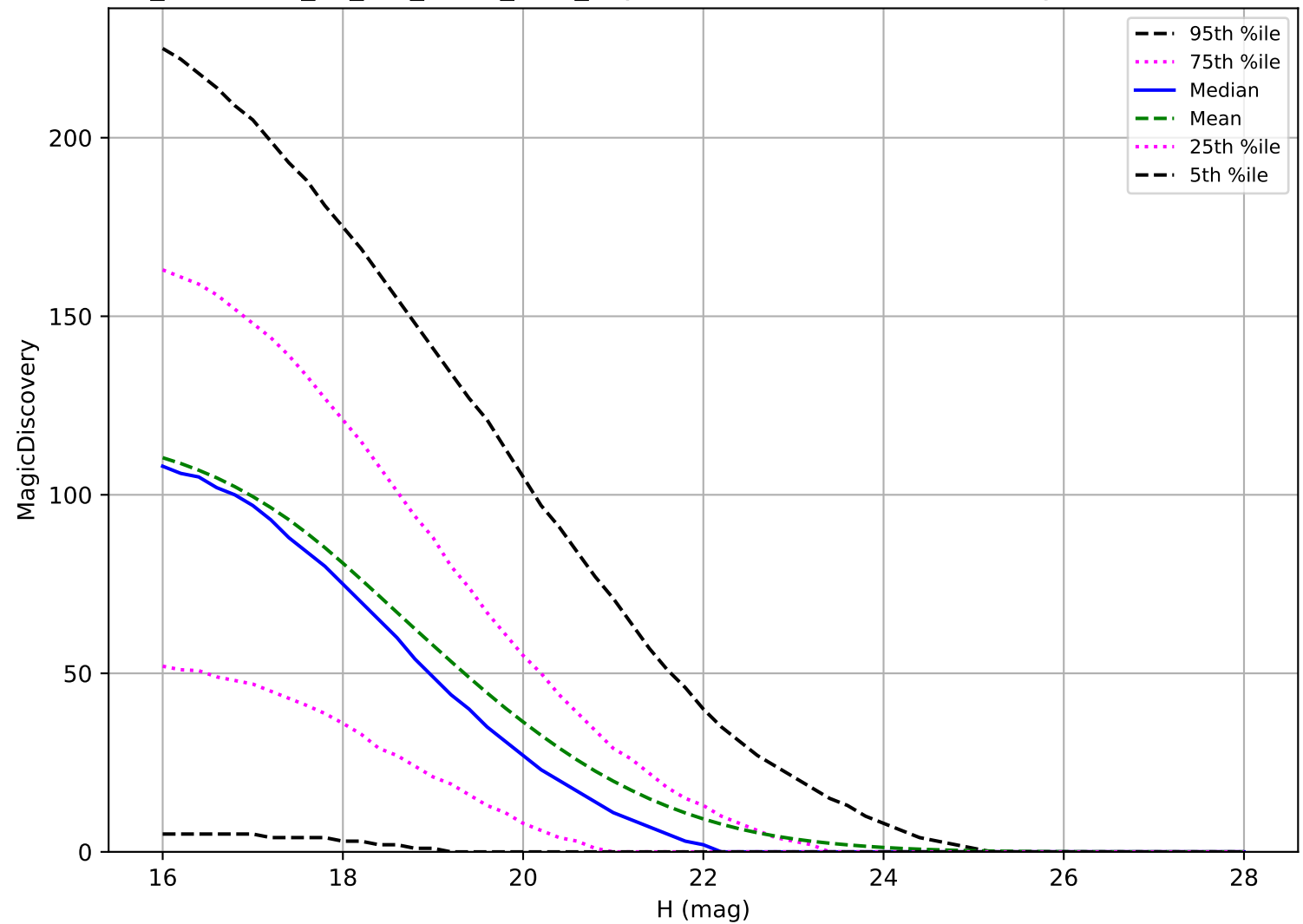
too_combined_no_nss_s10.0_v3.4_10yrs: NEO 6 detections in 60 nights detection loss
