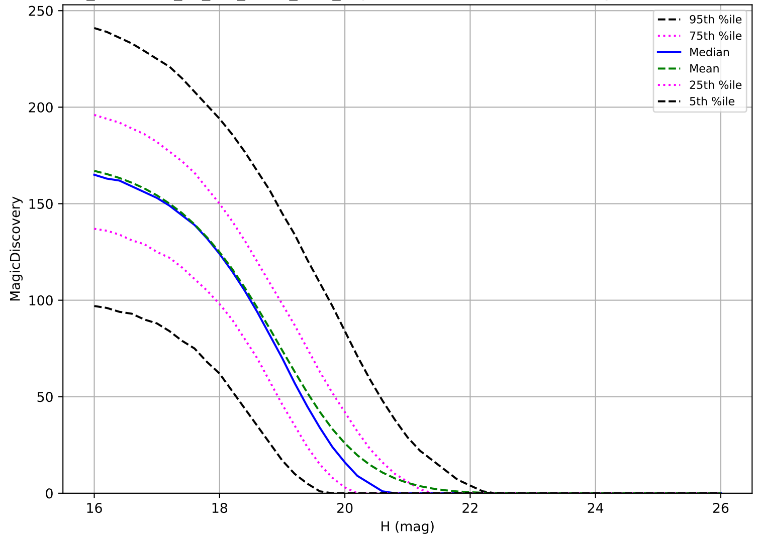
too_combined_no_nss_s10.0_v3.4_10yrs: MBA 6 detections in 60 nights detection loss
