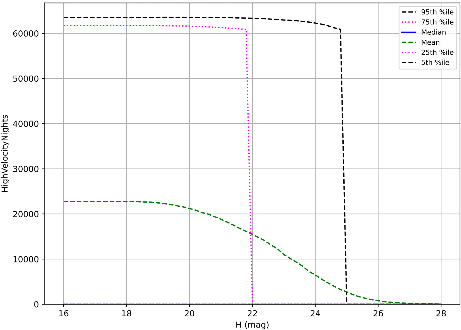
too_combined_no_nss_s10.0_v3.4_10yrs: NEO High velocity pair detection loss
