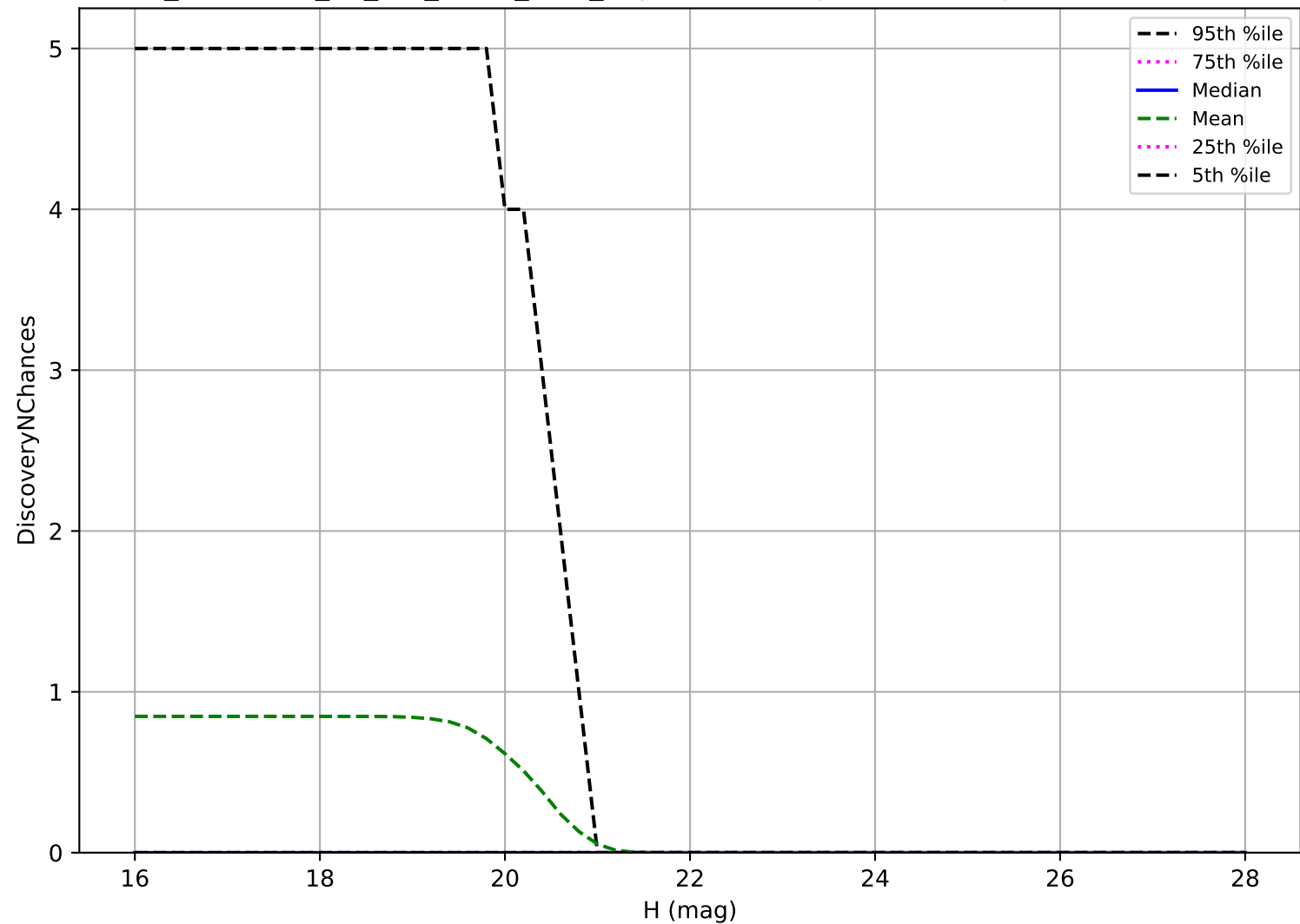
too_combined_no_nss_s10.0_v3.4_10yrs: Vatira 3 pairs in 15 nights detection loss
