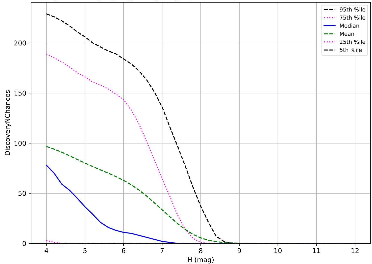
too_combined_no_nss_s10.0_v3.4_10yrs: TNO 3 pairs in 15 nights detection loss
