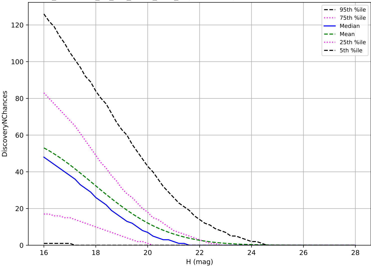
too_combined_no_nss_s10.0_v3.4_10yrs: PHA 3 pairs in 15 nights detection loss
