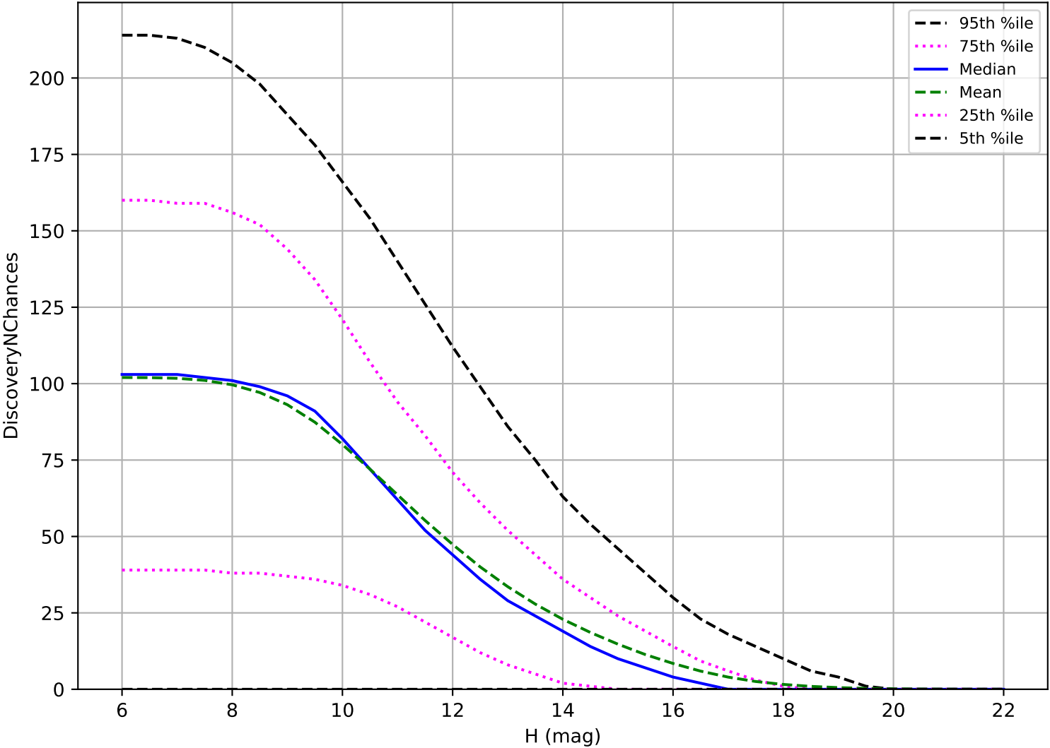
too_combined_no_nss_s10.0_v3.4_10yrs: OCC_r5 3 pairs in 15 nights detection loss
