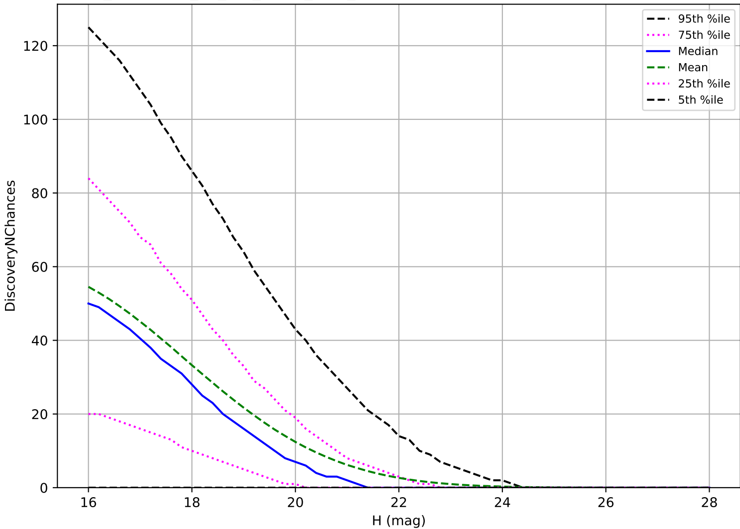
too_combined_no_nss_s10.0_v3.4_10yrs: NEO 3 pairs in 15 nights detection loss
