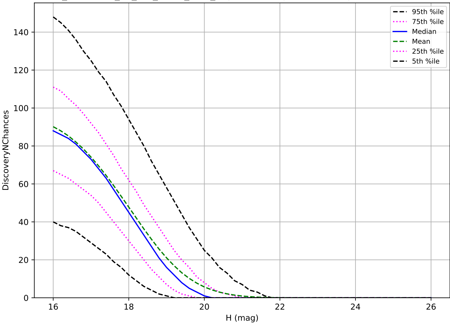
too_combined_no_nss_s10.0_v3.4_10yrs: MBA 3 pairs in 15 nights detection loss
