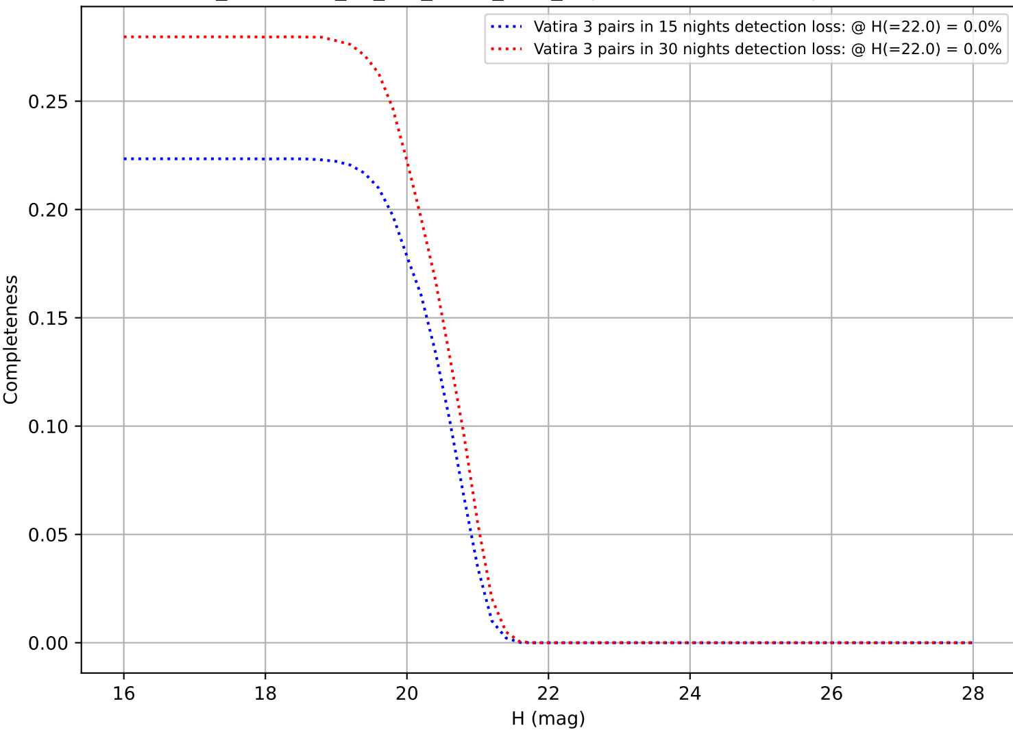
too_combined_no_nss_s10.0_v3.4_10yrs: DifferentialCompleteness
