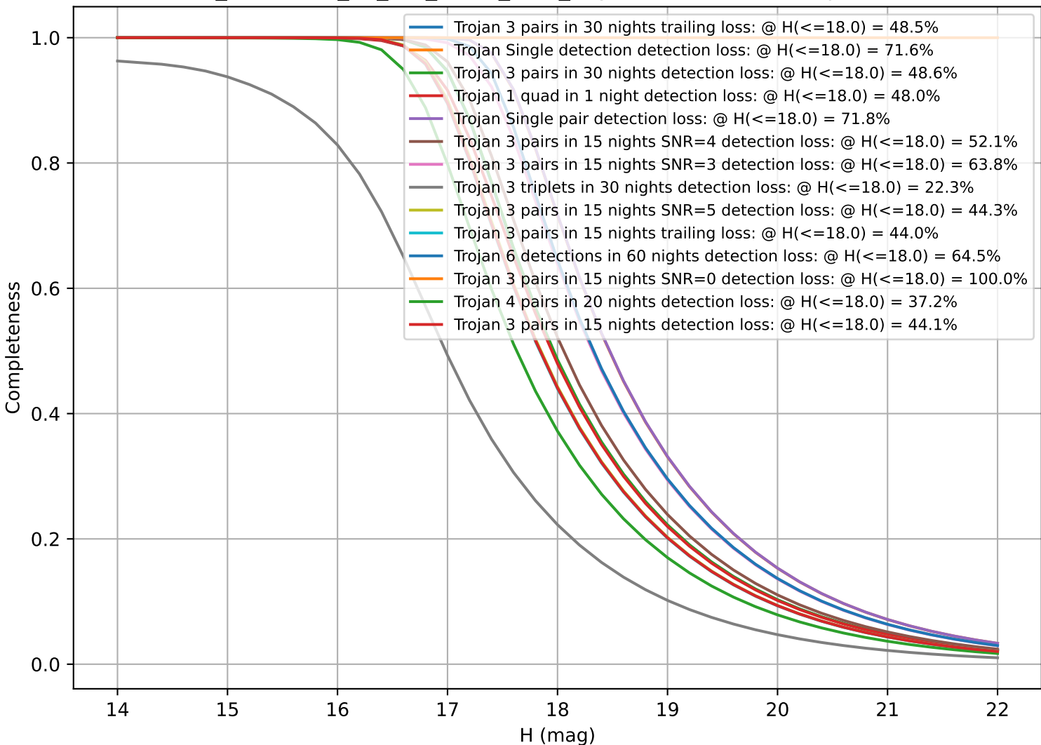
too_combined_no_nss_s10.0_v3.4_10yrs: CumulativeCompleteness
