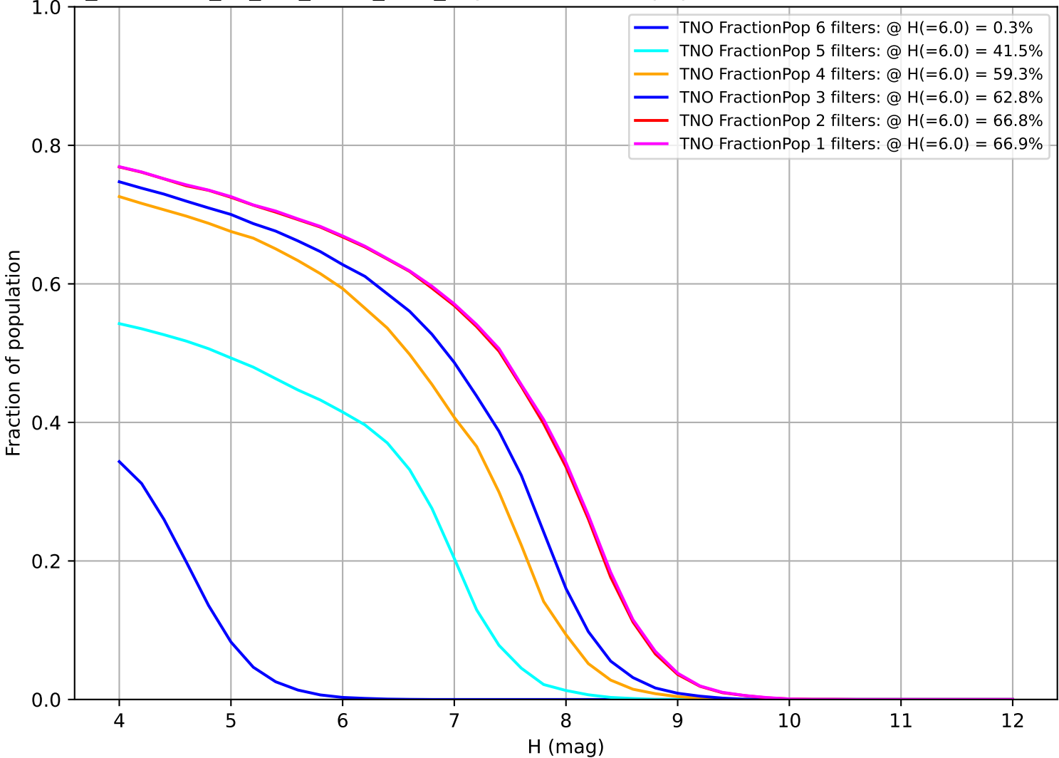
too_combined_no_nss_s10.0_v3.4_10yrs: Fraction of population with colors in X filters TNO
