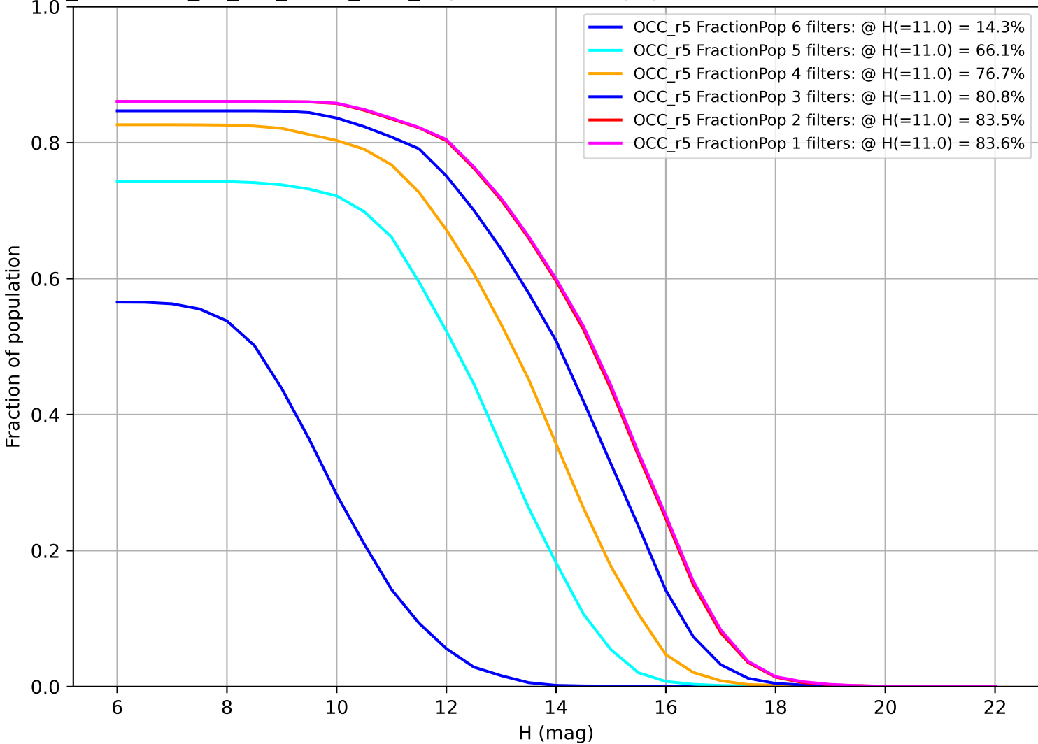
too_combined_no_nss_s10.0_v3.4_10yrs: Fraction of population with colors in X filters OCC_r5
