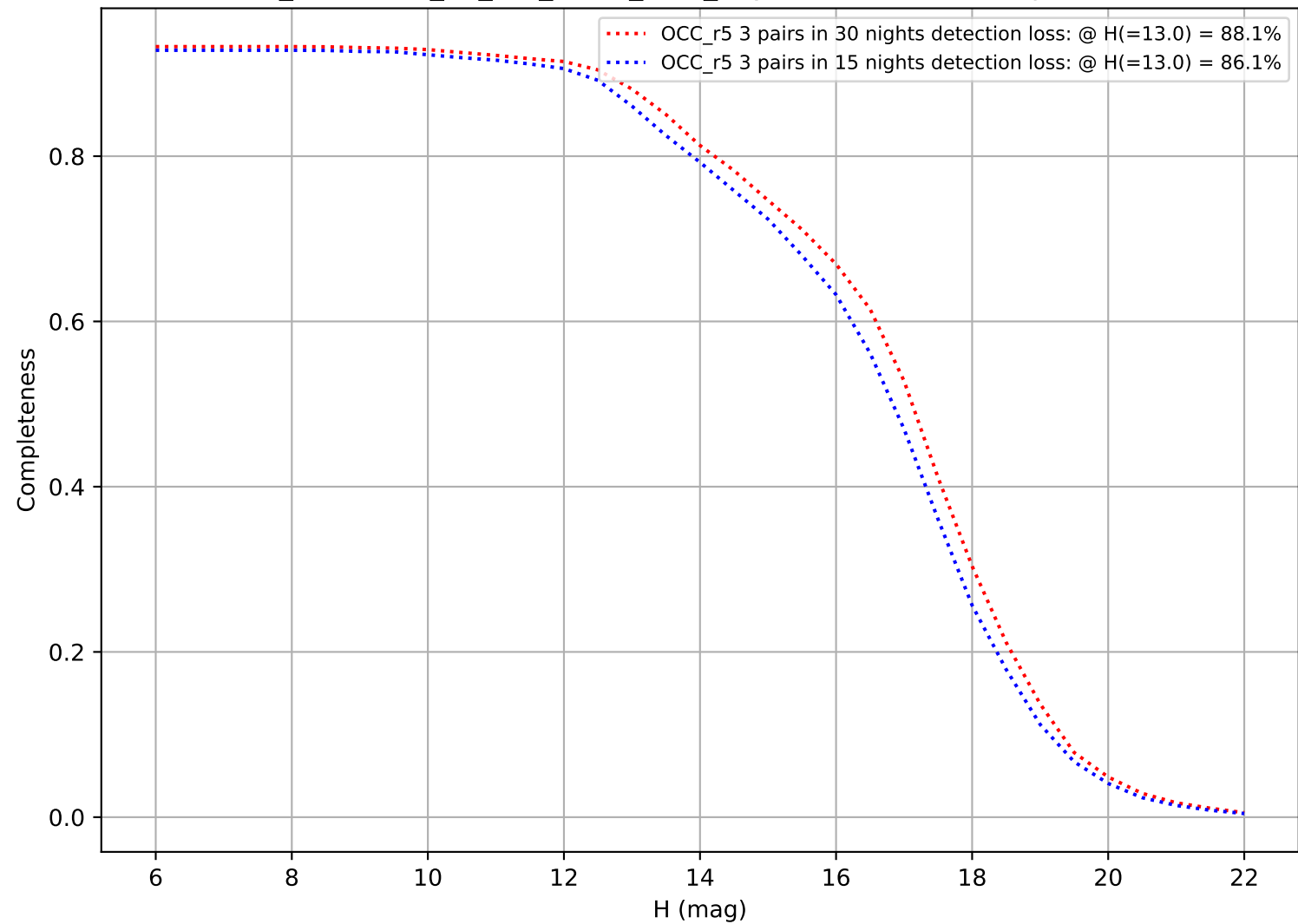
too_combined_no_nss_s10.0_v3.4_10yrs: DifferentialCompleteness
