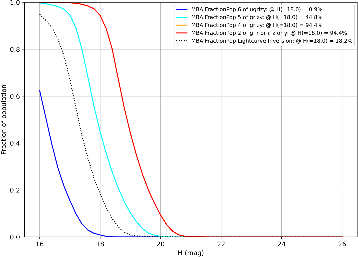
too_combined_no_nss_s10.0_v3.4_10yrs MBA
